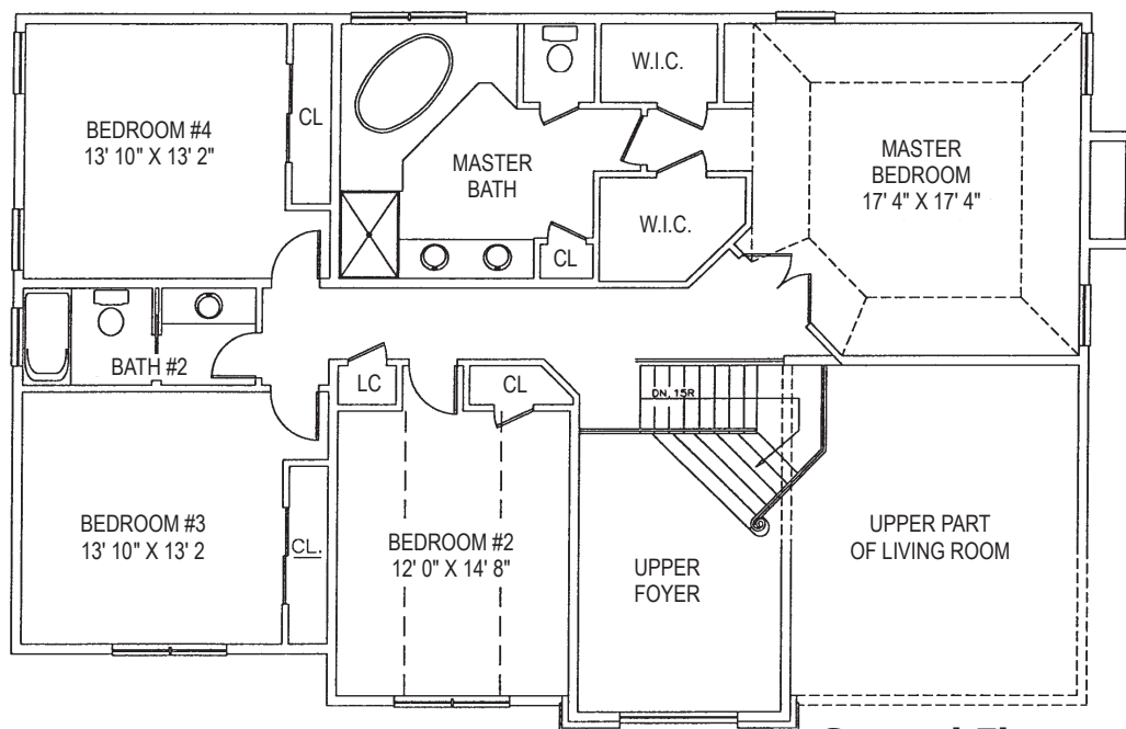
Second Floor
